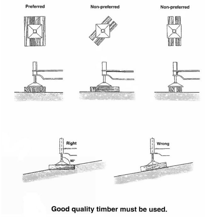
Figure 5 – Timber Packing Under Stabilizers
